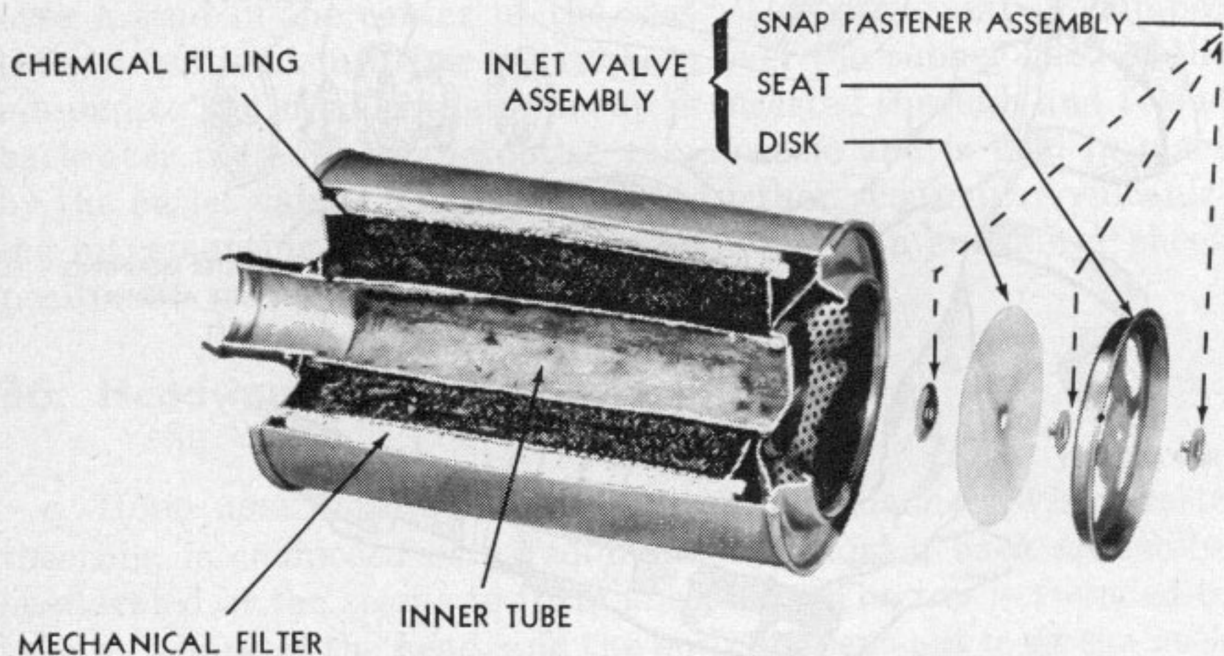
Figure 27. Service canister M10A1.
